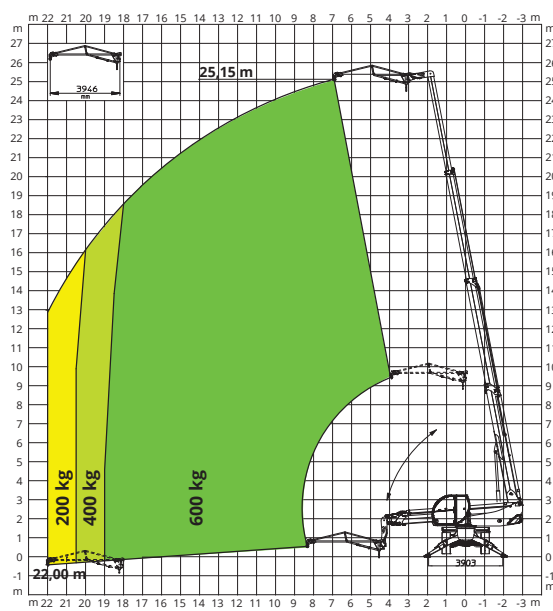
JIB 600 kg
